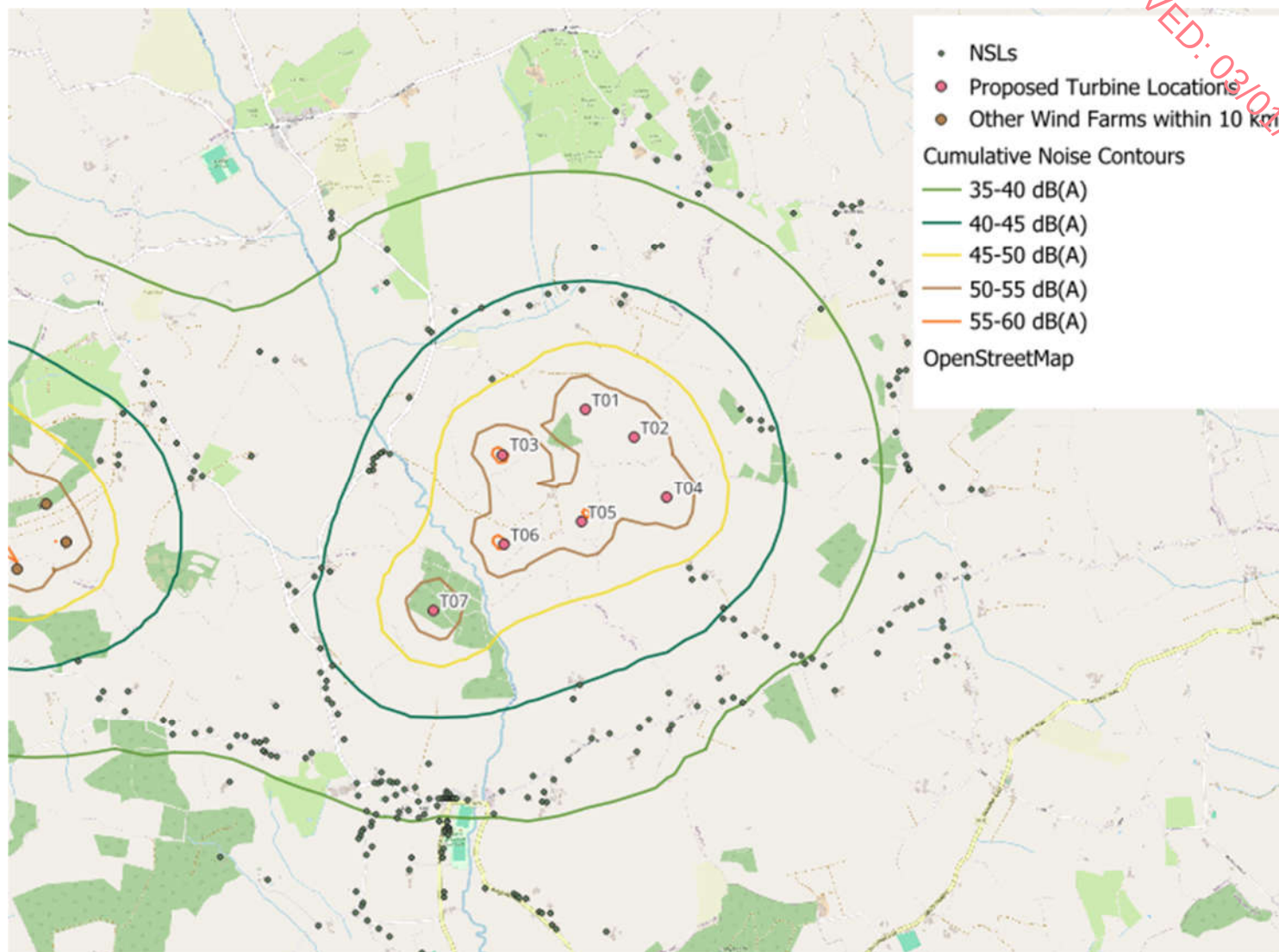
Figure 1 Cumulative Predicted Noise Contours
